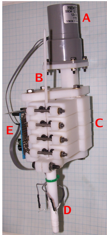
Figure 4. The first RepRap polymer transport mechanism.
