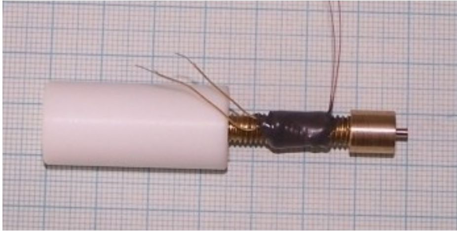
Figure 8. The first melt-chamber and nozzle design. The small squares are 1 mm.
